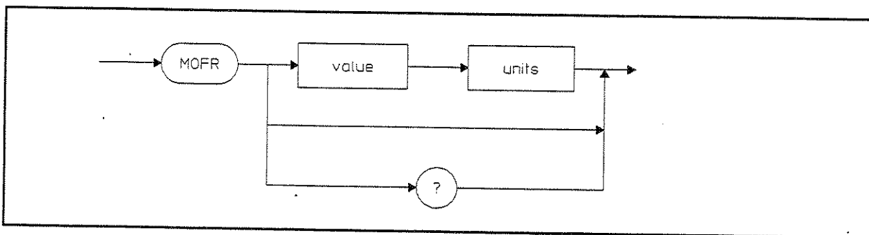
Figure 2-30. MOFR Syntax Diagram
